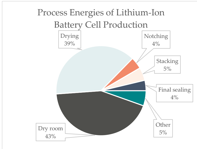
Figure 6. Circle diagram with different sources' energy contributions to the total cell production and battery pack assembly energy. Data from Yuan et al. (2017). The processes included in 'other' are: mixing, coating, calendaring, welding & sealing, LiPF 6 (electrolyte) filling, and pre-charging. It is clear here that running dry room equipment and NMP-drying are significantly larger contributors to process energy use than the sources.
